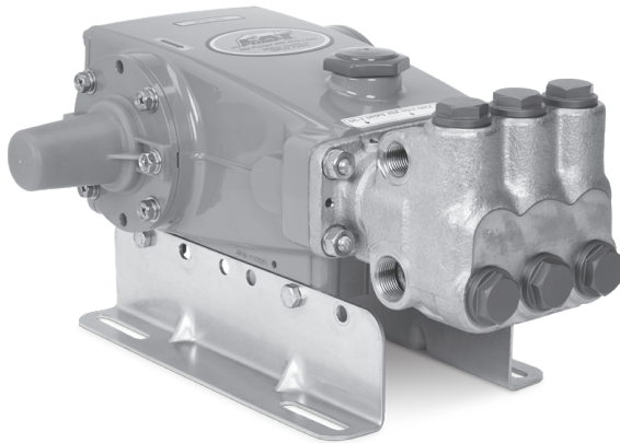
Model 1751 Shown (Shaft protector included rails sold separately)
