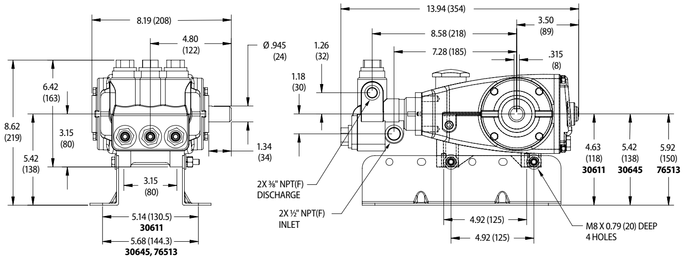
Models 56, 56HS
